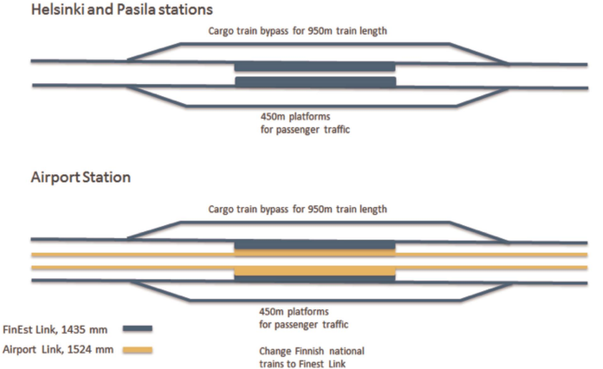
Figure 5.5 Schematic picture of station layout with cargo train bypasses
