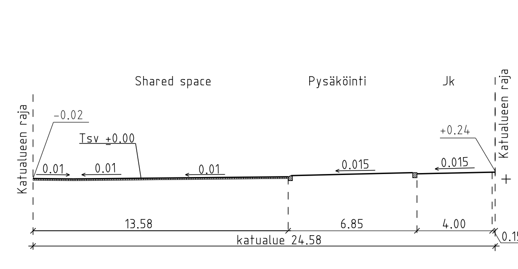
SHARED SPACE H-H
